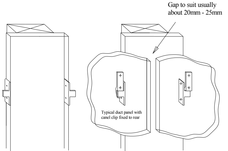
Typical drawing showing MIDDLE shadow panel & duct panel clip arrangement
