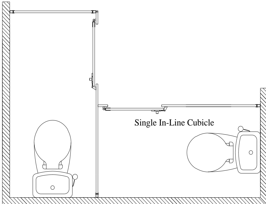
Corner In-Line Cubicle
